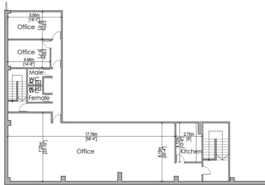
First Floor Plan Gross Internal Area (Excluding Staircase): Office: 185 sq m / 1,991 sq ft
