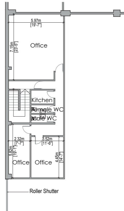
First Floor Plan Gross Internal Area (Excluding Staircase): Office: 91 sq m / 980 sq ft
